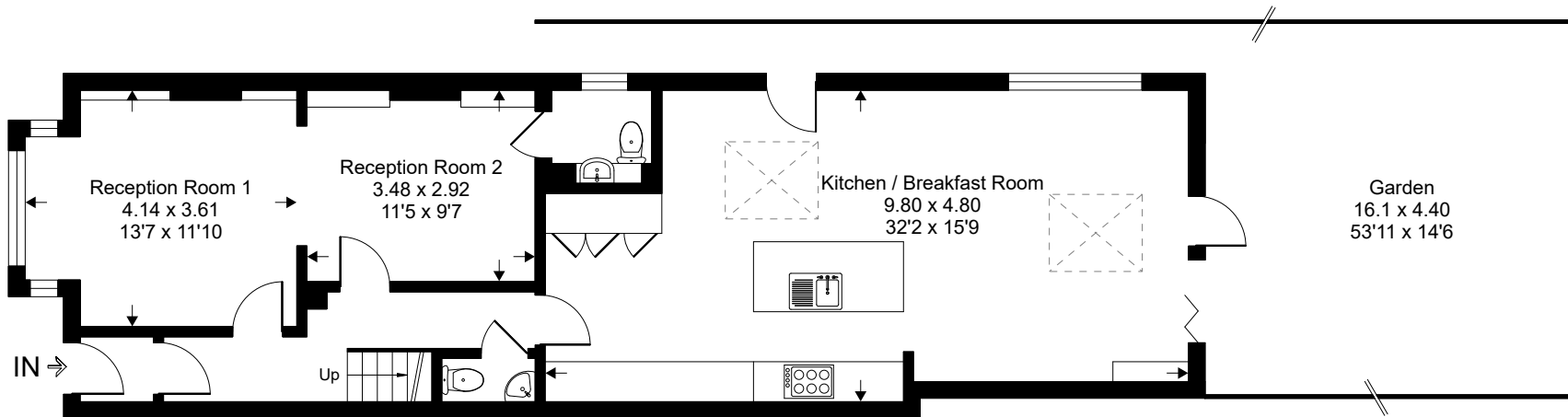
Ground Floor
