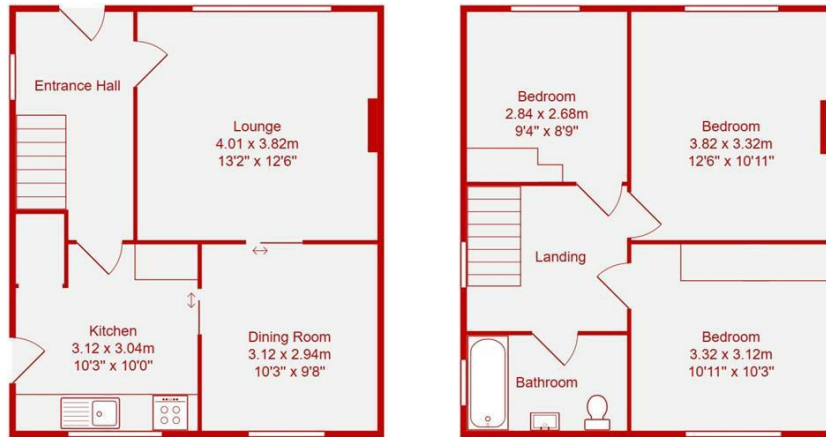
Ground Floor Area: 43.0 m 2 ... 463 ft 2
